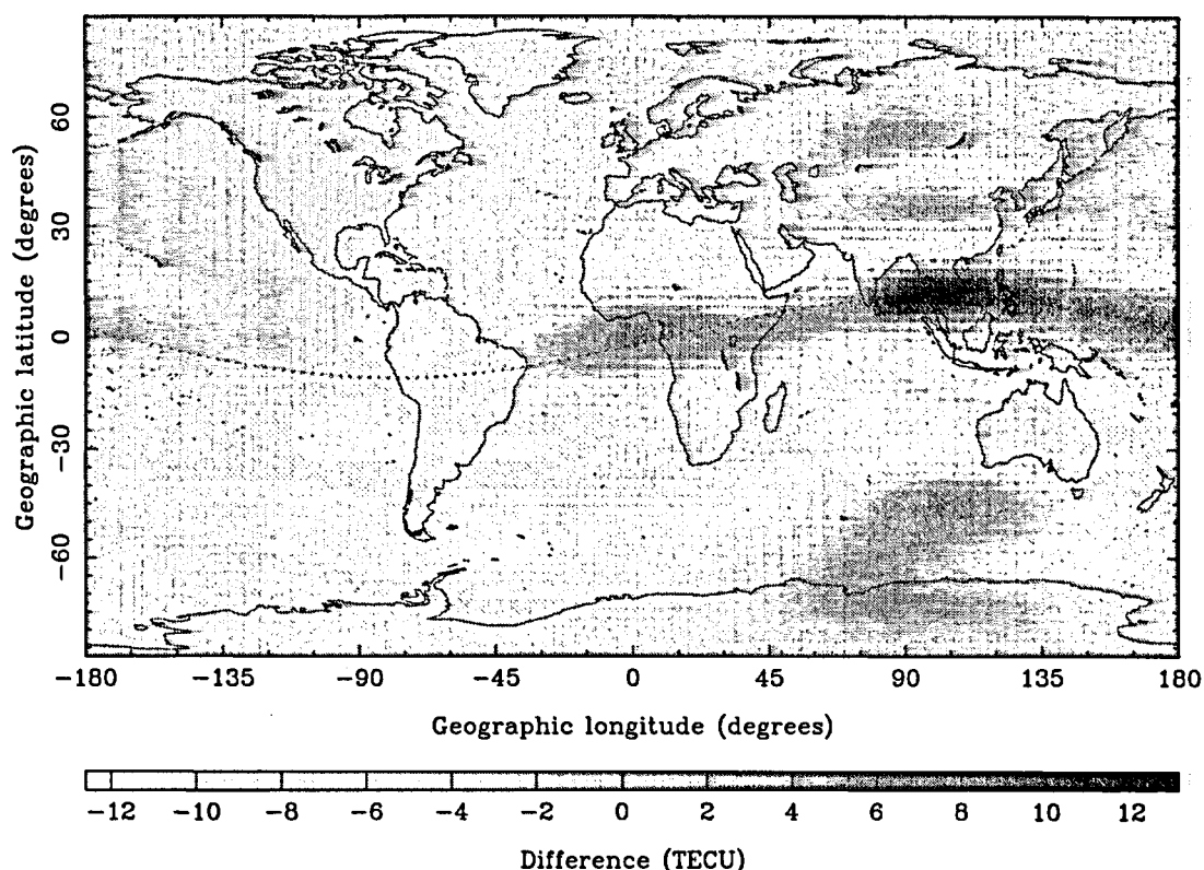
Figure 6.12: Global map of the difference between COD(Z1) and JPL GIMs referring to 13:00 UT each, from August 28, 1998 to January 31, 1999.
