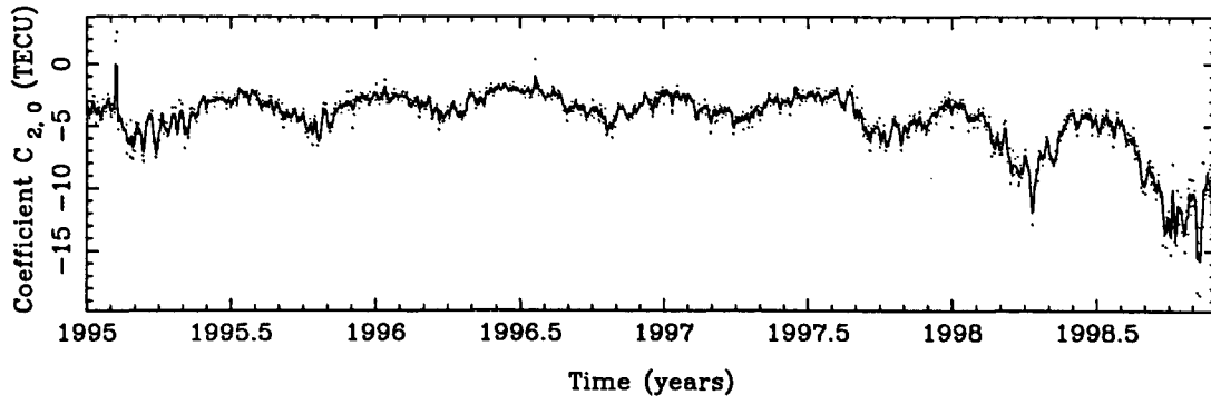
Figure A.5: SH coefficient \tilde{C}_{2,0} .
