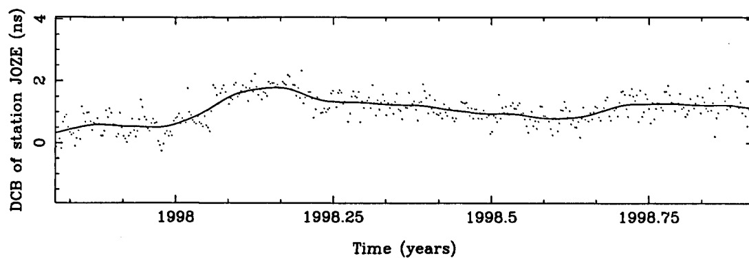
Figure B.32: DCB of the station JOZE (Jozefoslaw, Poland).
