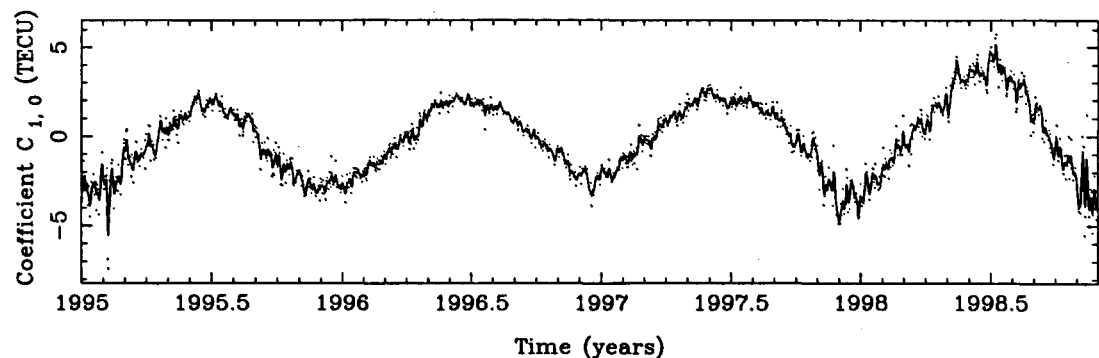
Figure A.2: SH coefficient \tilde{C}_{1,0} .
