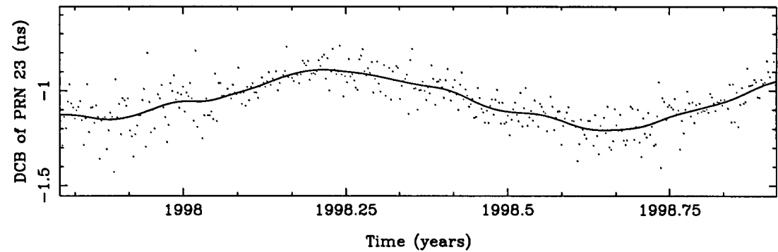
Figure 4.34: DCB of PRN 23.
