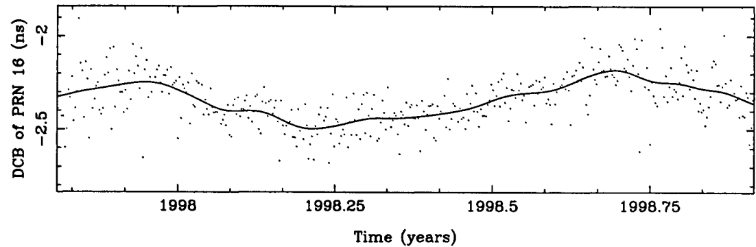
Figure B.14: DCB of PRN 16.
