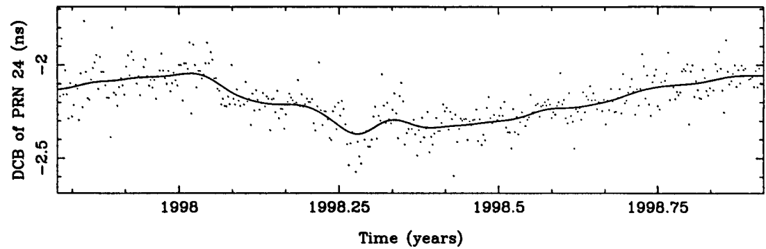
Figure B.21: DCB of PRN 24.
