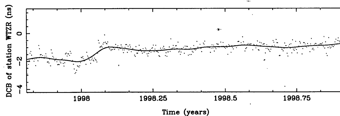
Figure B.37: DCB of the station WTZR (Wettzell, Germany).
