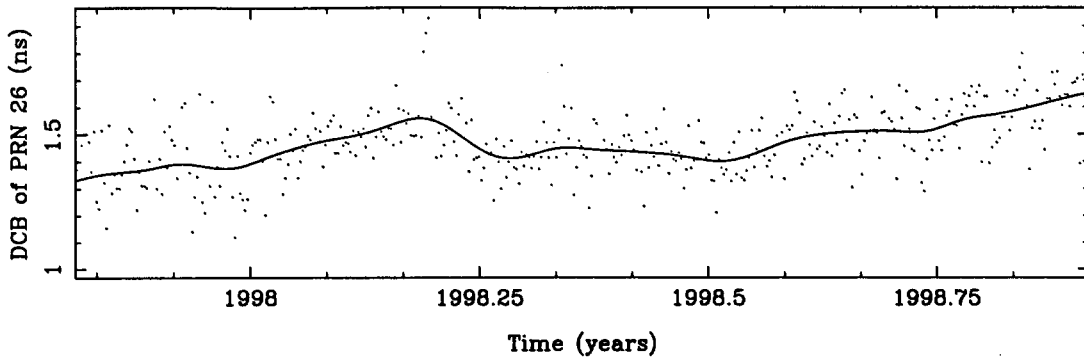
Figure B.23: DCB of PRN 26.
