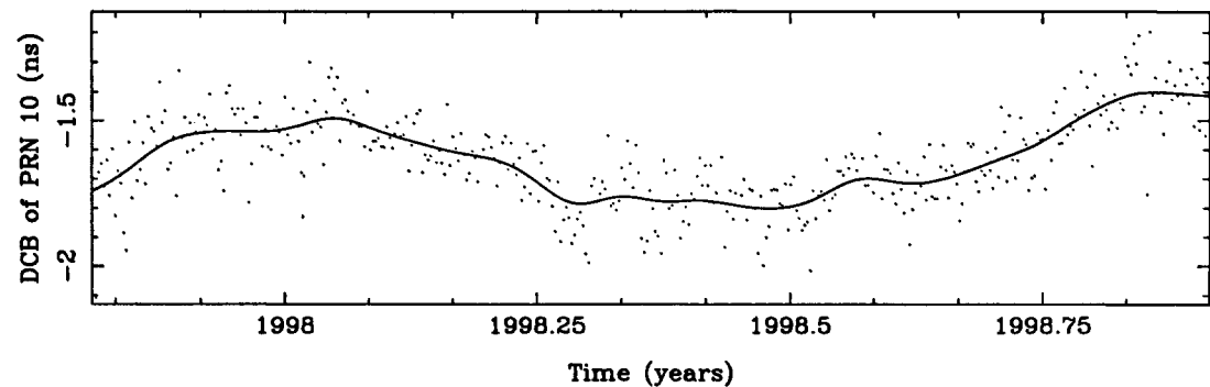
Figure B.10: DCB of PRN 10.
