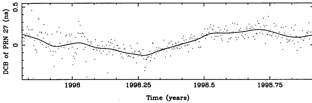
Figure B.24: DCB of PRN 27.
