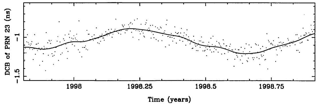
Figure B.20: DCB of PRN 23.
