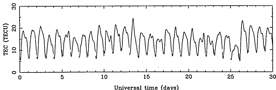
Figure 4.25: Daily TEC profiles evaluated at (\beta, \lambda) = (50^\circ, 7.5^\circ) , for June 1998.
