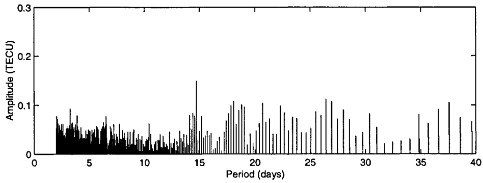
(b) Sine coefficient \tilde{S}_{1,1}
