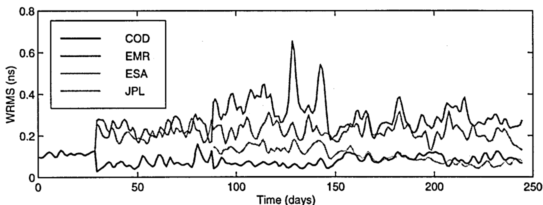
Figure 6.17: WRMS errors obtained from daily satellite DCB combinations, from June 1, 1998 to January 31, 1999.
