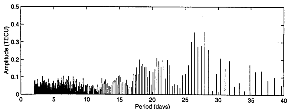
Figure 4.16: Amplitude spectrum of the mean TEC, for periods below 40 days.
