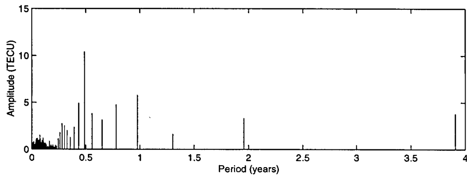
Figure 4.20: Amplitude spectrum of the maximum TEC.
