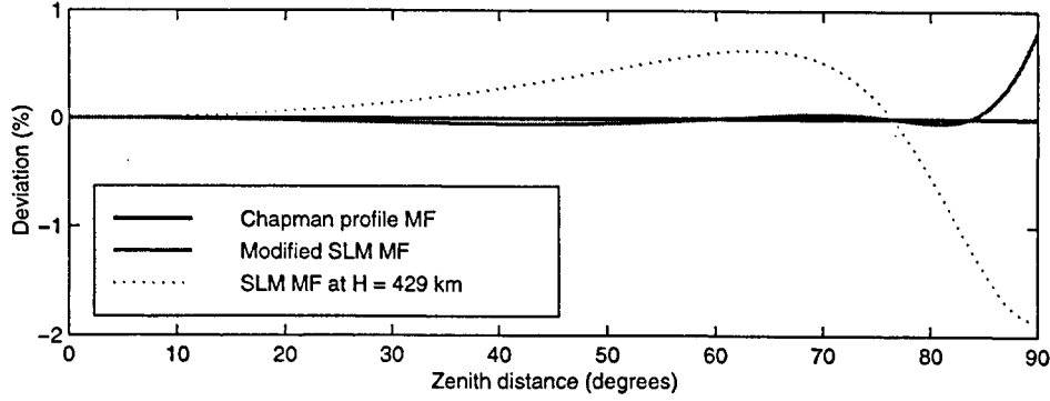
Figure 3.10: Deviation of the modified SLM mapping function with respect to the reference Chapman profile mapping function.
