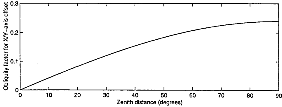
Figure 4.37: Obliquity factor for the X/Y-axis satellite antenna offset.
