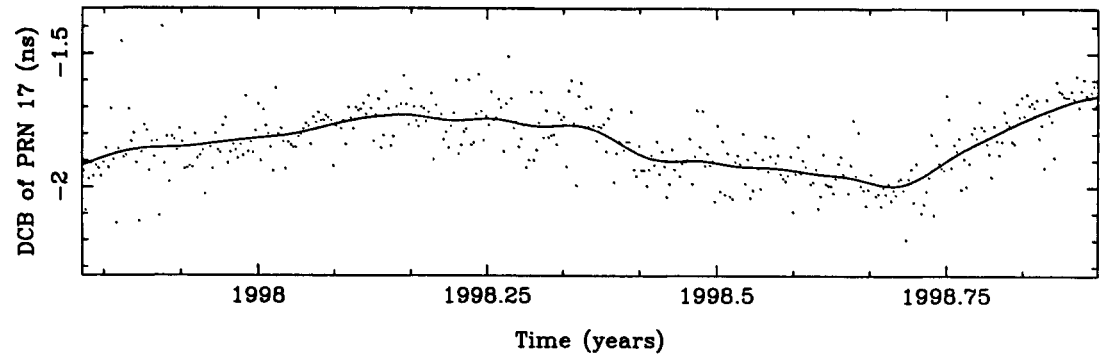
Figure B.15: DCB of PRN 17.
