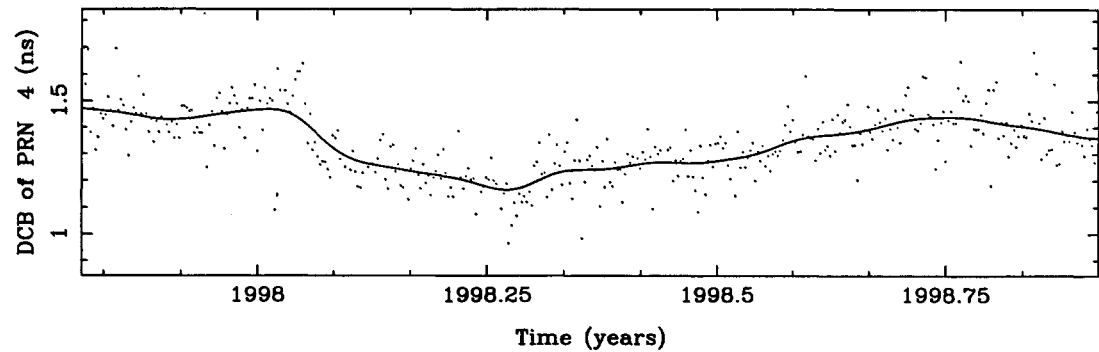
Figure B.4: DCB of PRN 4.
