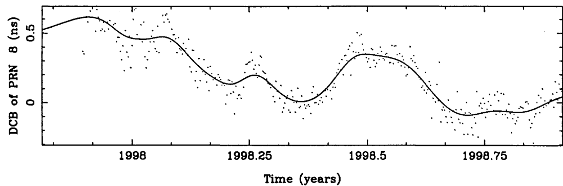
Figure B.8: DCB of PRN 8.
