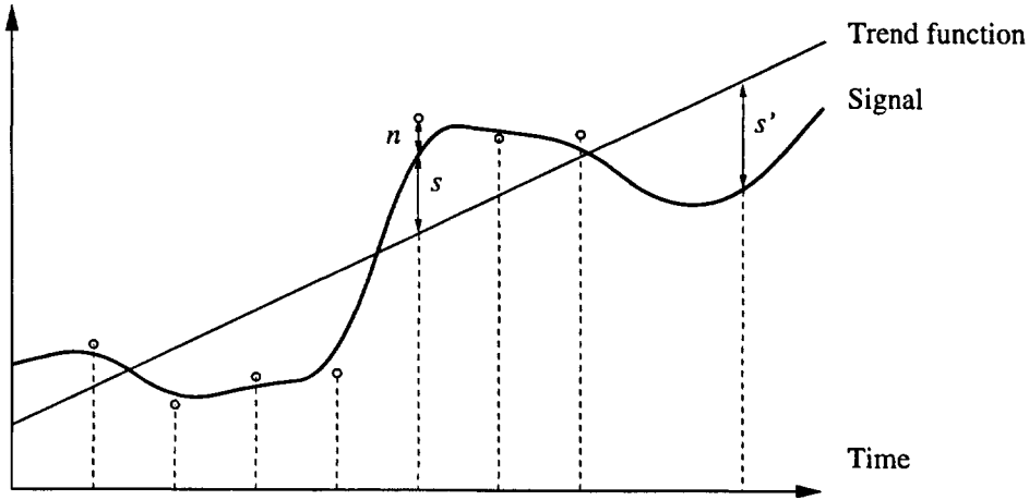
Figure 5.1: Components of the least-squares collocation: noise n , signal s , predicted signal s' , and trend function.
