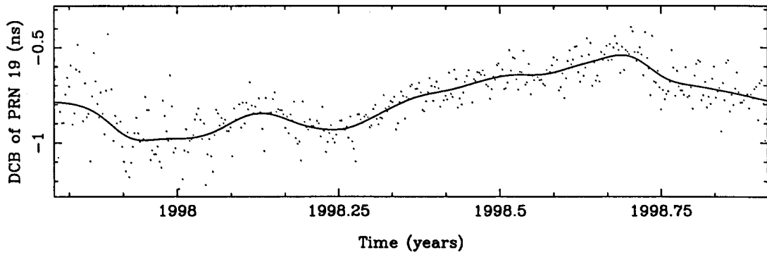
Figure B.17: DCB of PRN 19.
