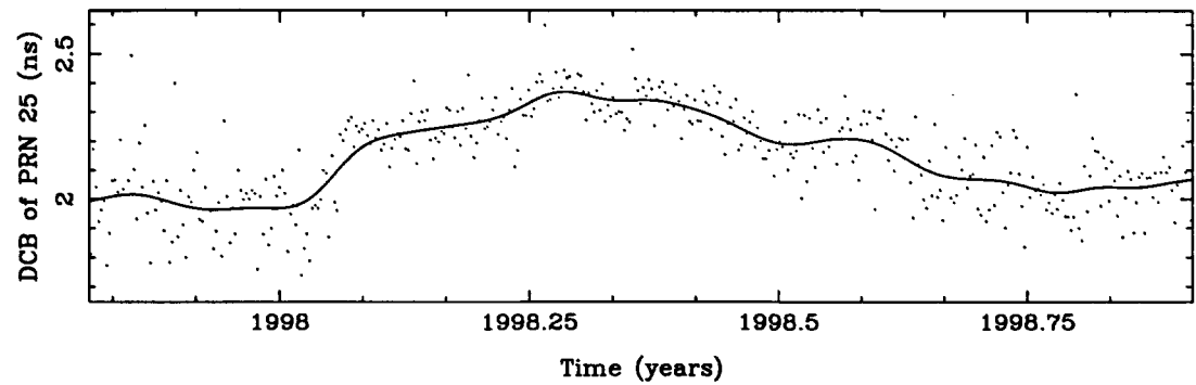
Figure B.22: DCB of PRN 25.
