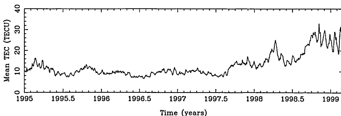
Figure 7.1: Mean vertical TEC of the Earth's ionosphere computed by CODE, from January 1995 to February 1999.
