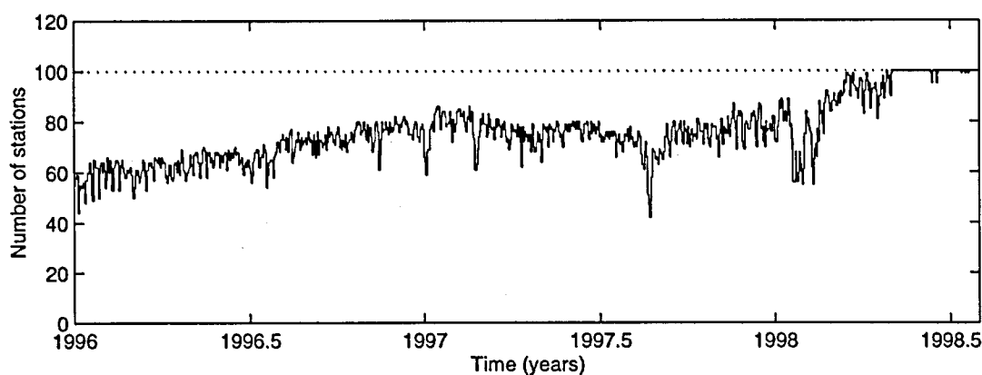
Figure 4.3: Number of IGS stations daily processed by CODE, from January 1996 to July 1998.
