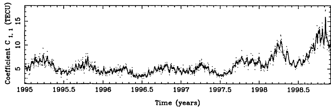
Figure A.3: SH coefficient \tilde{C}_{1,1} .
