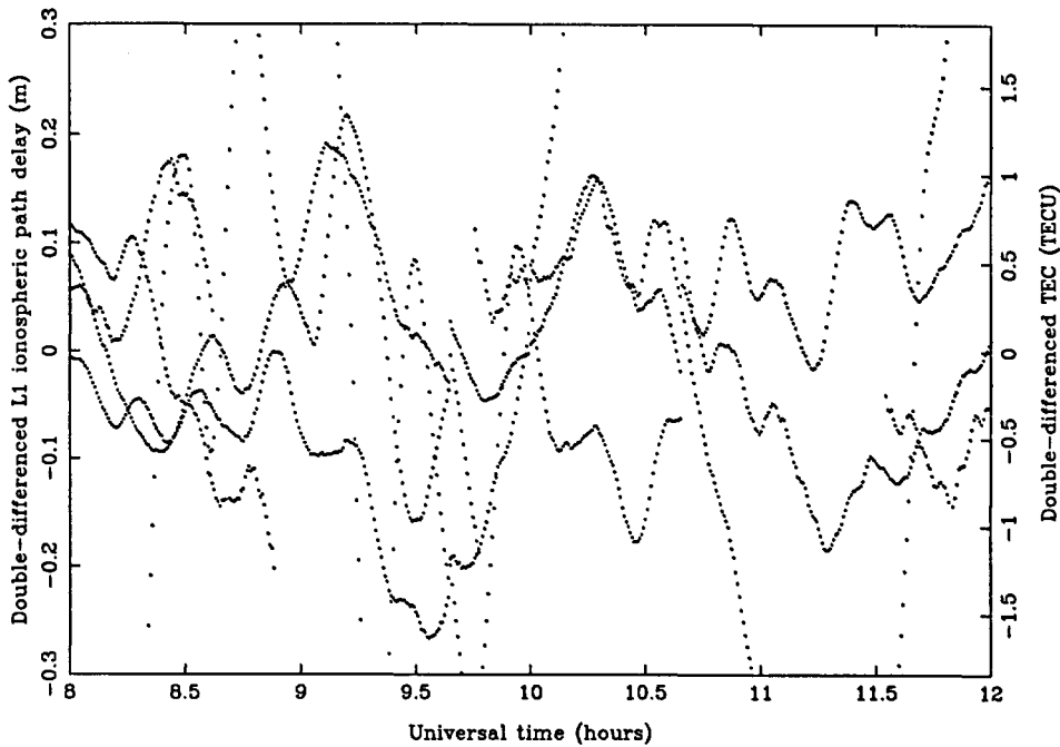
Figure 6.4: Medium-scale traveling ionospheric disturbances (MSTIDs) on the baseline Kootwijk-Wettzell, for January 25, 1994 (08:00 to 12:00 UT).
