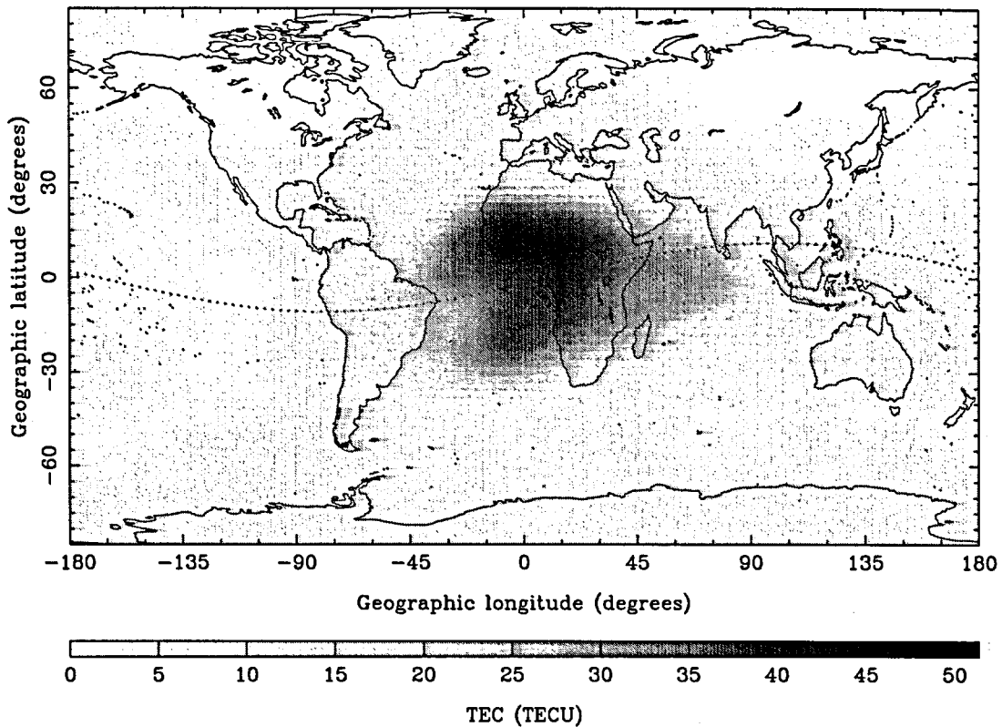
Figure 4.7: Global TEC on January 17, 1998 at 13:00 UT.
