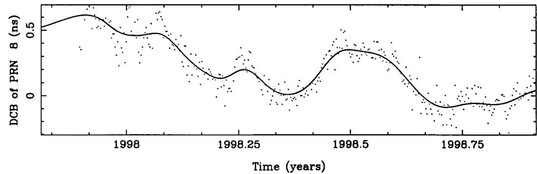
Figure 4.35: DCB of PRN 8.
