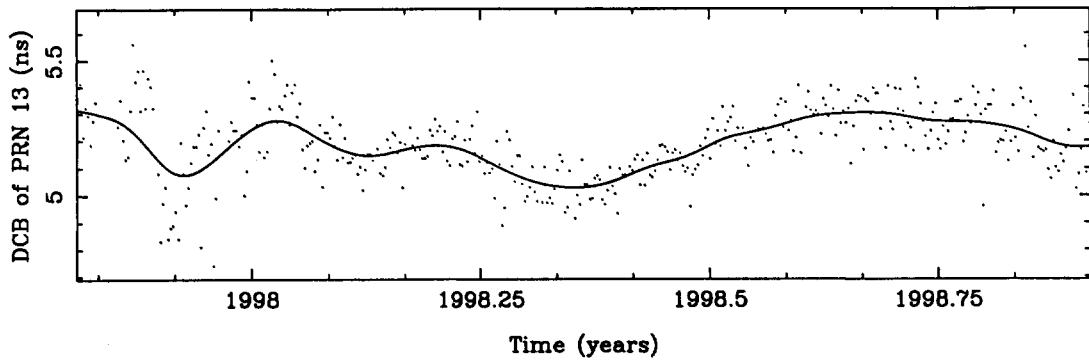
Figure B.11: DCB of PRN 13.
