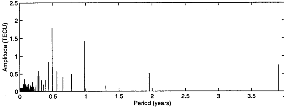
Figure 4.15: Amplitude spectrum of the mean TEC.
