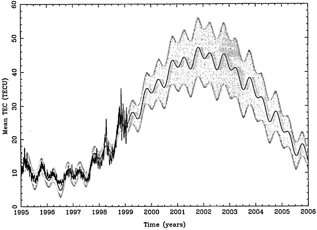
Figure 5.7: Mean TEC \tilde{C}_{0,0} and trend function \Psi(t) , fitted to 4 years of global TEC observations and extrapolated for the next 7 years.
