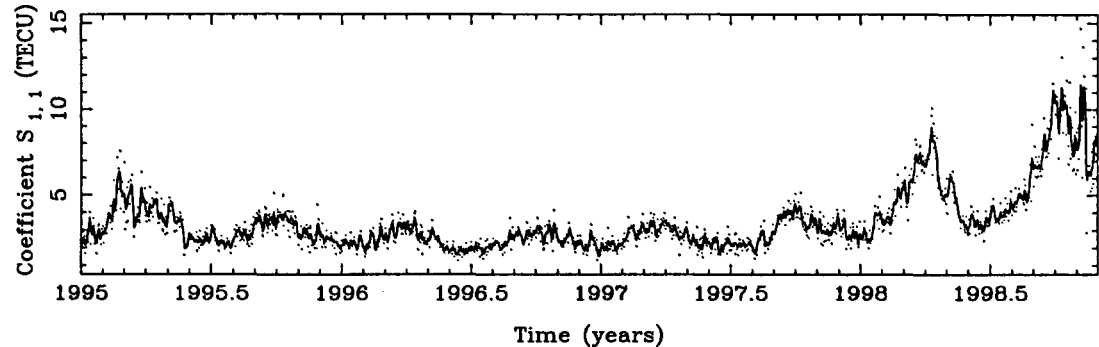
Figure A.4: SH coefficient \tilde{S}_{1,1} .
