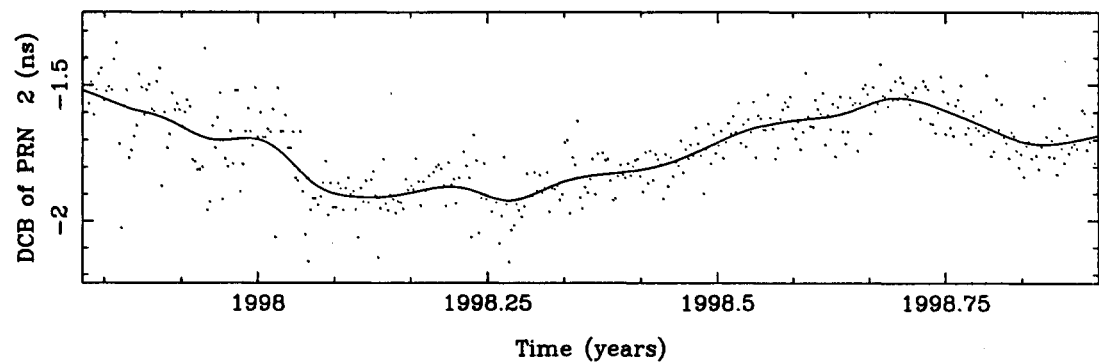
Figure B.2: DCB of PRN 2.
