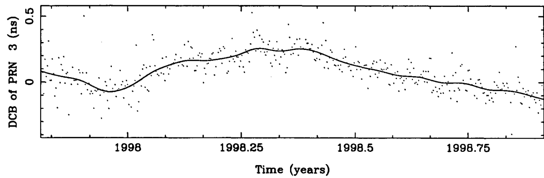
Figure B.3: DCB of PRN 3.
