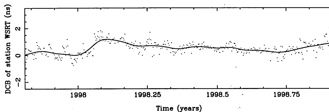
Figure B.36: DCB of the station WSRT (Westerbork Synthesis Radio Telescope, The Netherlands).
