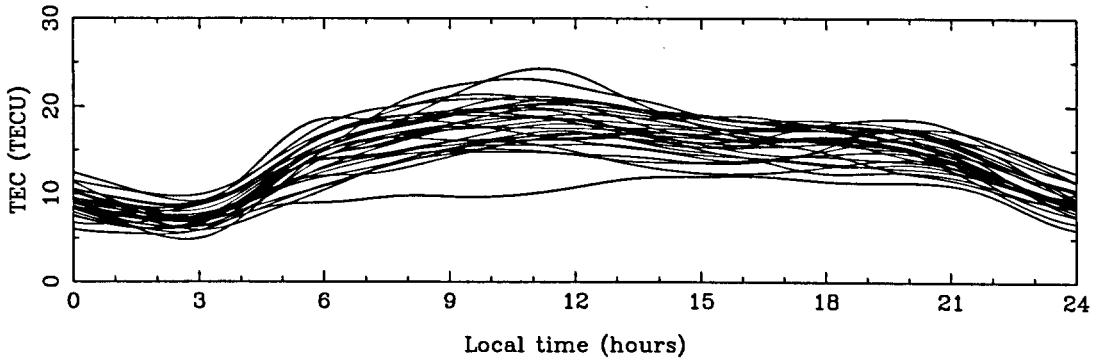
Figure 4.26: Daily TEC profiles evaluated at (\beta, \lambda) = (50^\circ, 7.5^\circ) as a function of local time, for June 1998.
