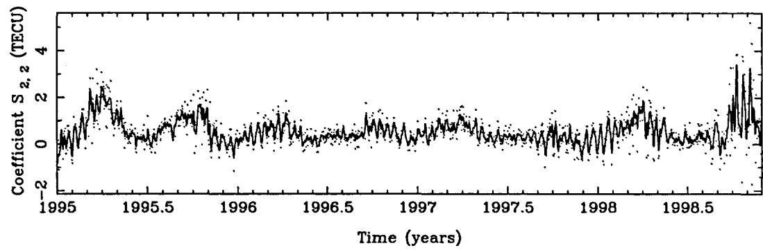
Figure A.9: SH coefficient \tilde{S}_{2,2} .
