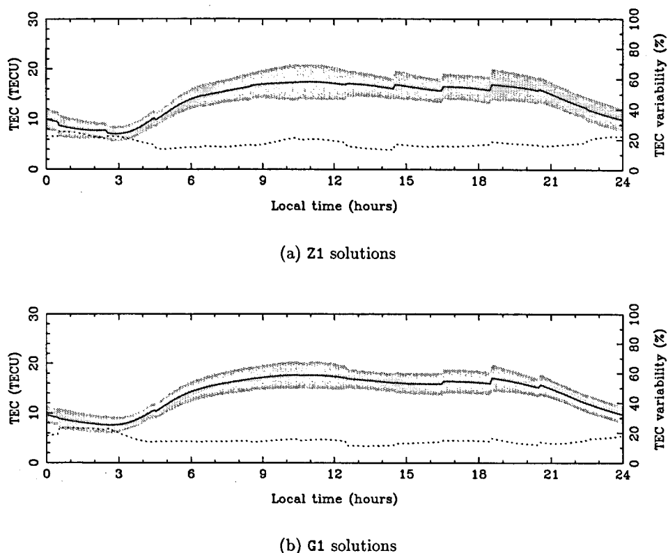
Figure 6.10: Day-to-day TEC variability at (\beta, \lambda) = (50^\circ, 7.5^\circ) derived from Z1 or G1 solutions of June 1998.
