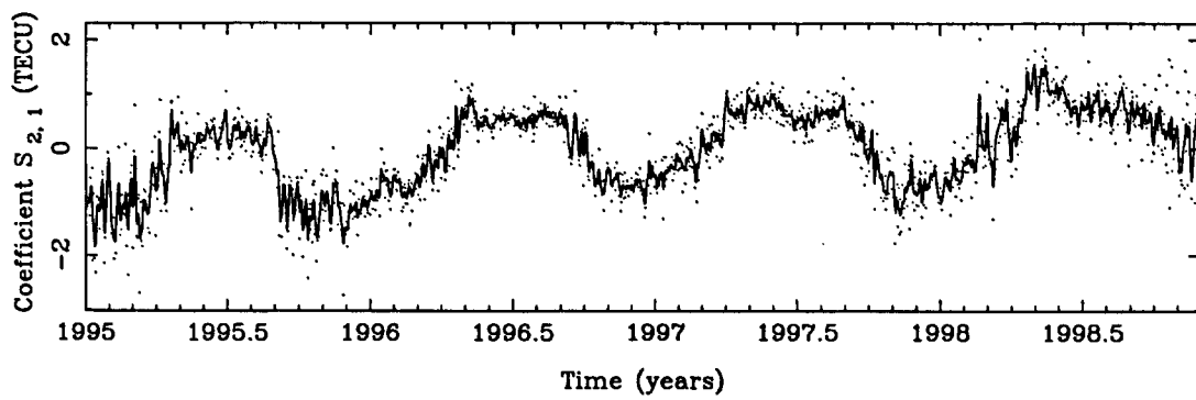
Figure A.7: SH coefficient \tilde{S}_{2,1} .
