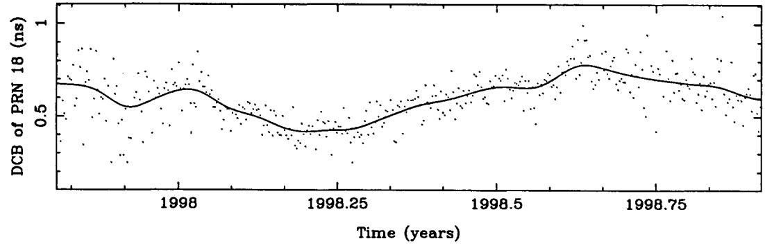
Figure B.16: DCB of PRN 18.
