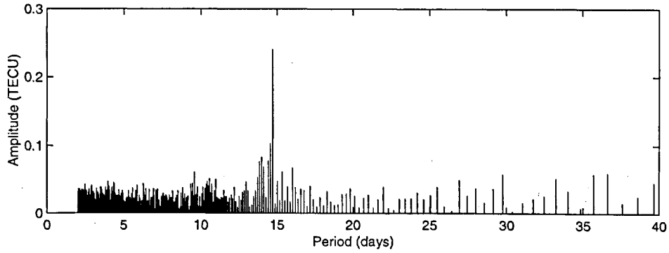
(a) Cosine coefficient \tilde{C}_{2,2}
