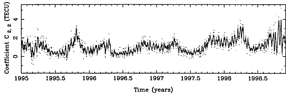
Figure A.8: SH coefficient \tilde{C}_{2,2} .
