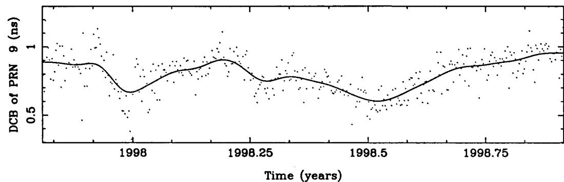
Figure B.9: DCB of PRN 9.
