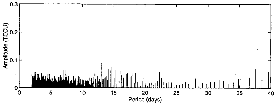
(b) Sine coefficient \tilde{S}_{2,2}
