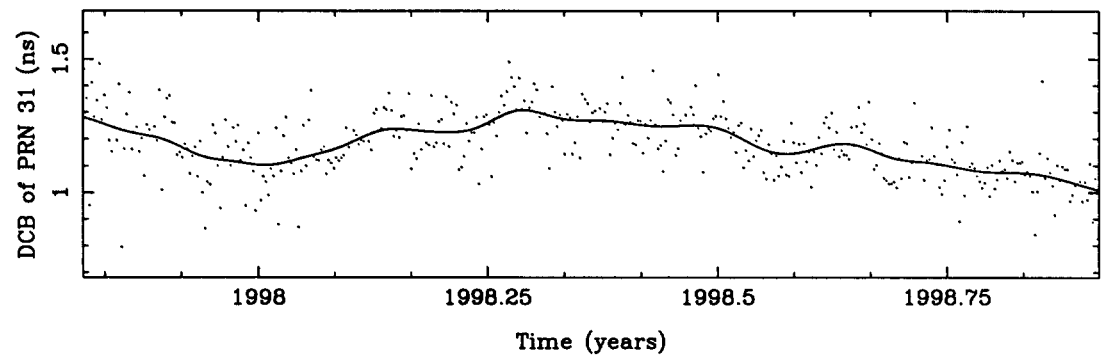
Figure B.27: DCB of PRN 31.
