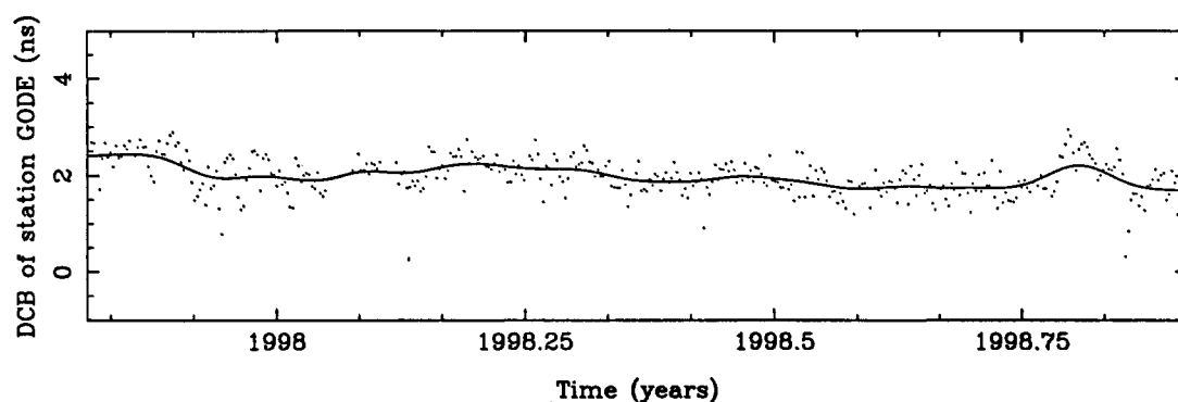
Figure B.31: DCB of the station GODE (Goddard Geophysical and Astronomical Observatory, Greenbelt, USA).
