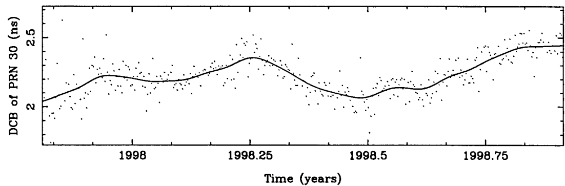
Figure B.26: DCB of PRN 30.
