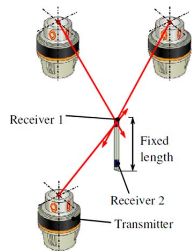
Figure 6.2 iGPS scale determination, by Schmitt et al. (2010), origin from Nikon
