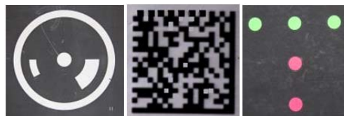
Figure 4.4 Three examples of coded targets used for point identification and camera calibration
